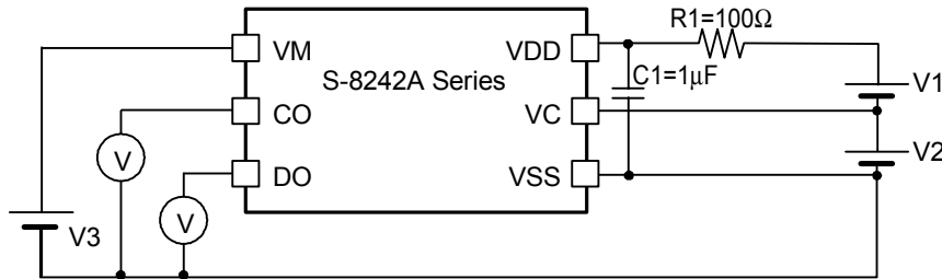
Figure 5 Test circuit 1
