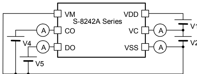
Figure 8 Test circuit 4
